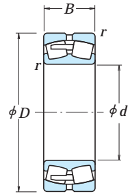
Cylindrical Bore
